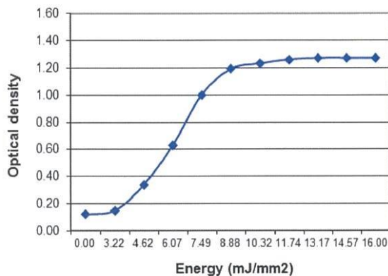
Dynamic sensitivity
